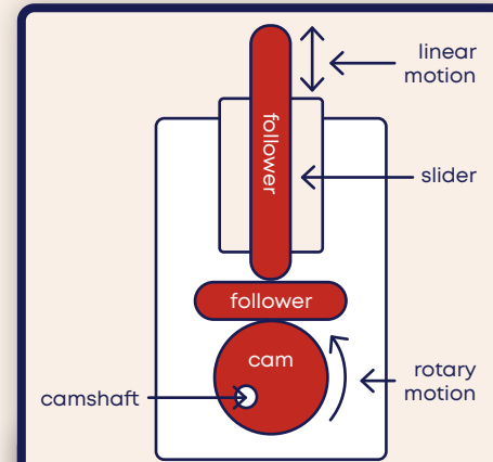
cross-sectional diagram showing a cams mechanism
